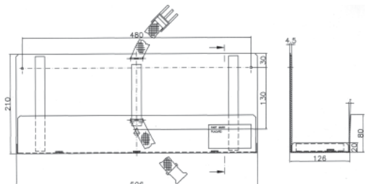
PNR 6240-05-001 • Bracket
